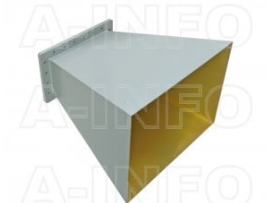
LB-1150-10-A Standard Gain Horn Antenna 0.64-0.96GHz 10dB Gain Rectangular Waveguide Interface
