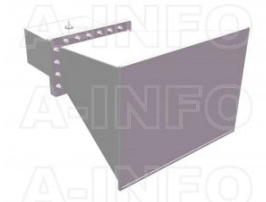
LB-1150-10-C-SFSPO Standard Gain Horn Antenna 0.64-0.96GHz 10dB Gain SMA Female
